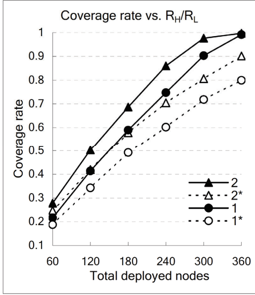
Fig. 7. Coverage rate of Test Case II
