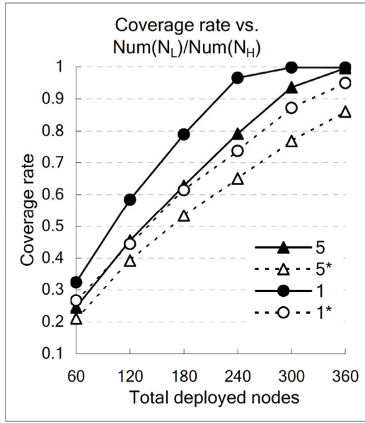
Fig. 5. Coverage rate of Test Case I
