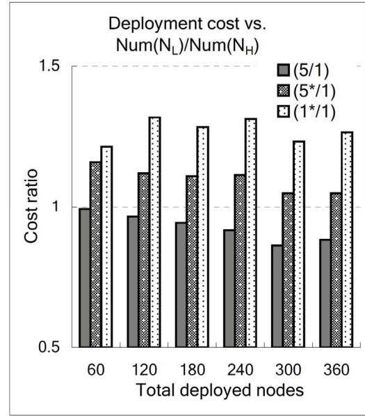
Fig. 6. Deployment cost of Test Case I
