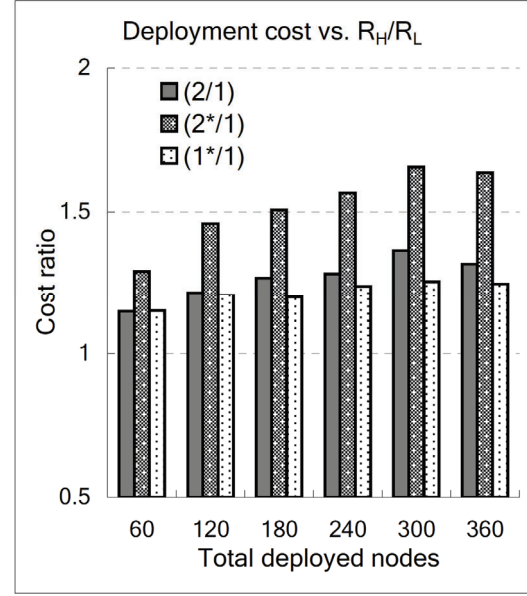
Fig. 8. Deployment cost of Test Case II
