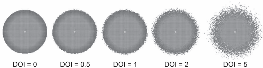
Fig. 1. The radio propagation range under different DOI
