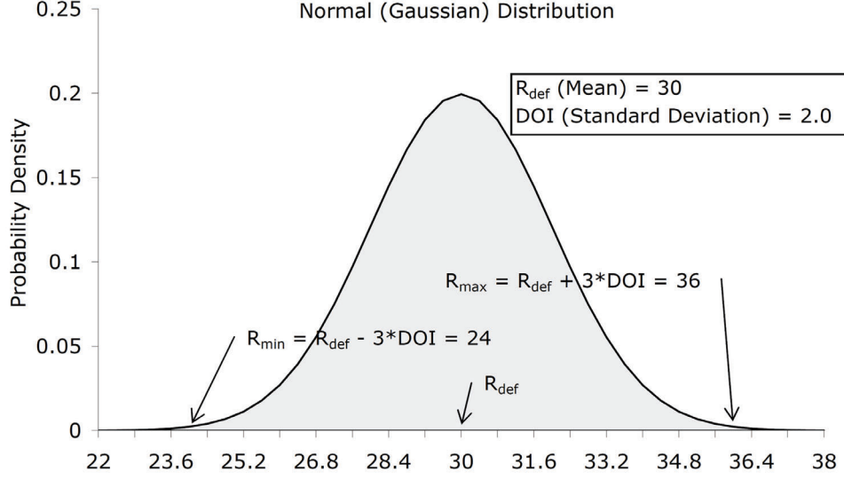
Fig. 2. The relationship between R_{\text{def}} , R_{\text{min}} , and R_{\text{max}}
