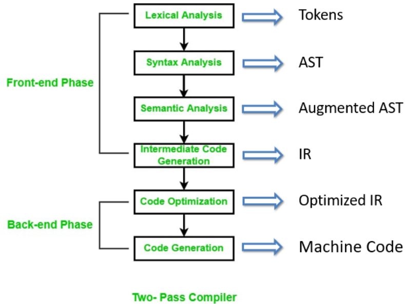
Figure 1: Compiler Structure
